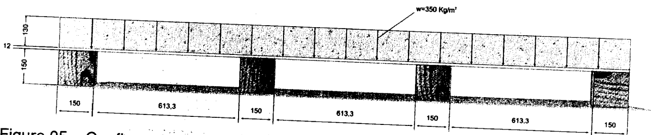
Figure 05 – Configuration layout.
